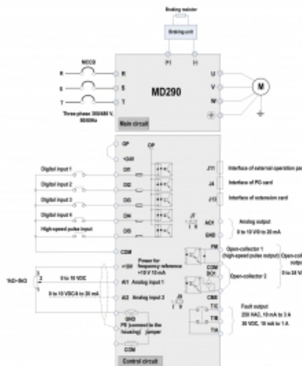
Figure 4-12 Wiring of the MD290 of three-phase 380 to 480 V (30G/110P to 110G/132P)
