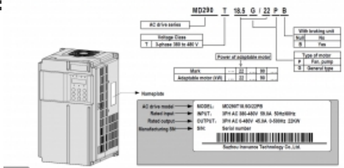
Figure 2-1 Nameplate and designation rules of the MD290
