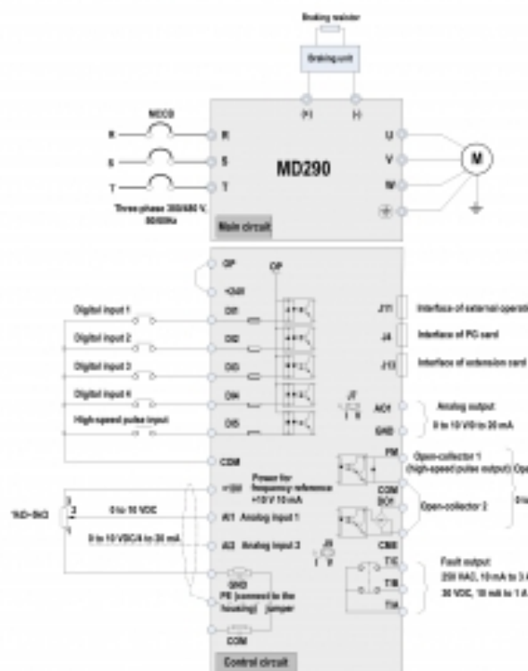
Figure 4-12 Wiring of the MD290 of three-phase 380 to 480 V (30G/110P to 110G/132P)
