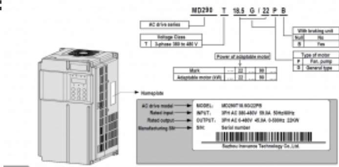
Figure 2-1 Nameplate and designation rates of the MD290
