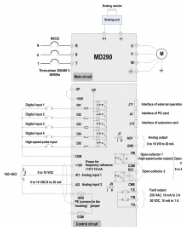
Figure 4-12 Wiring of the MD290 of three-phase 380 to 480 V (30G/118P to 118G/132P)
