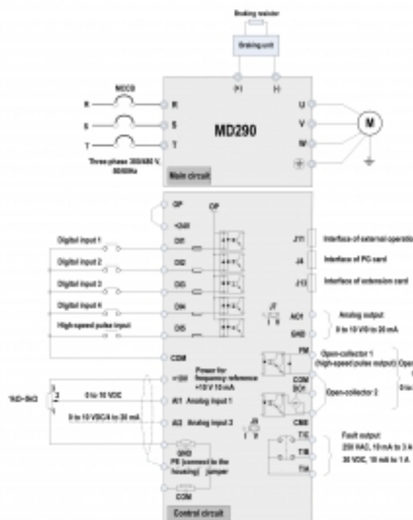
Figure 4-12 Wiring of the MD290 of three-phase 380 to 480 V (90G/118P to 110G/132P)
